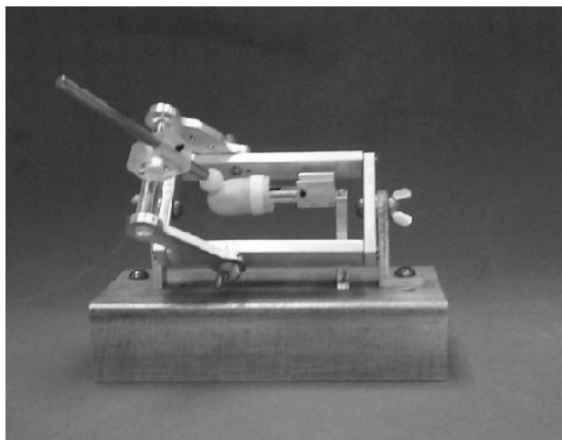
Figure 8: Indenter apparatus.
