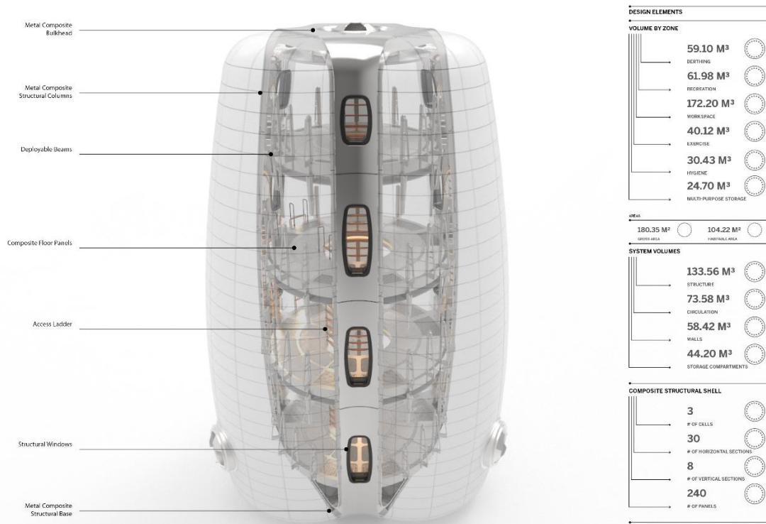
Figure 9. Habitat System Calculations. Axonometric
