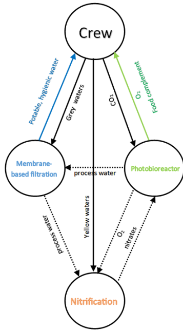
Figure 8. A schematic representation of the potential Life Support System concept for the early stage of a Moon settlement
