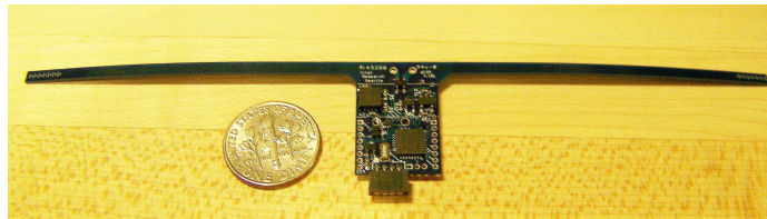
Figure 2-3: WISP Version 4.1
