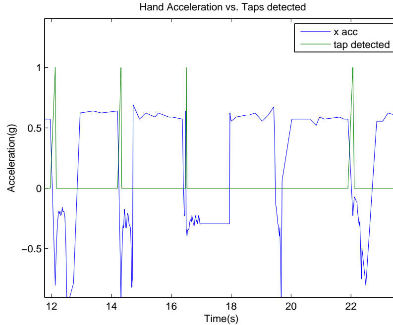
Figure 4-26: Finger tap on hard surface
