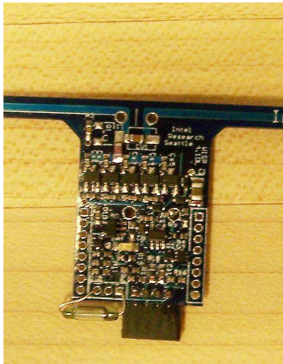
Figure 4-16: The WISP with reed switch attached
