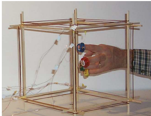
Figure 1-7: Paradiso and Hsaio's RF musical keyboard
