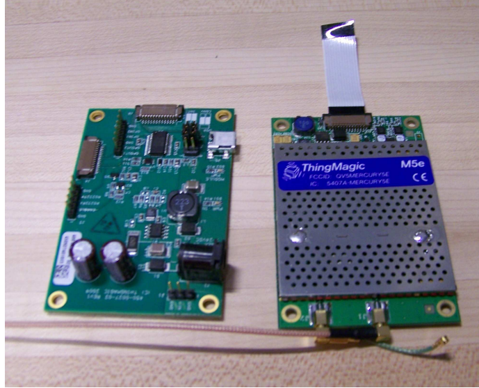
Figure 4-15: M5e Modules and Power/Interface Board
