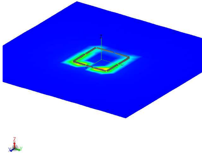
Figure 4-9: Near field patterns of a simulated square loop
