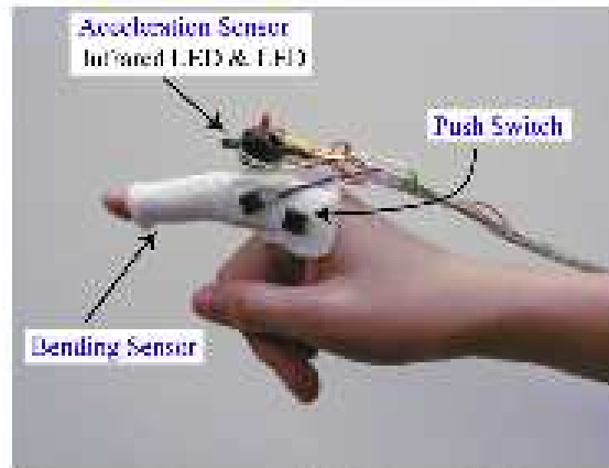
Figure 1-1: Ubi-finger prototype
