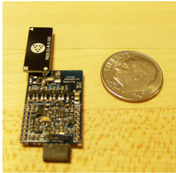
Figure 4-13: WISP with Fractus Chip Antenna
