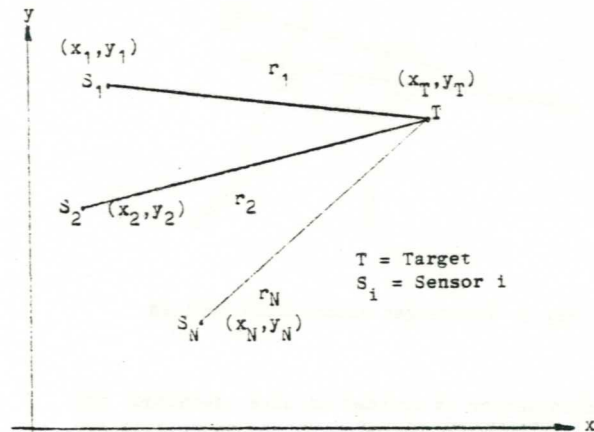
Fig. 2: Target-sensor geometry
