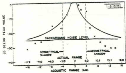
Fig. 18. Detection data for U-8 (altitude = 300 m, 0 dB = 68 dBa).
