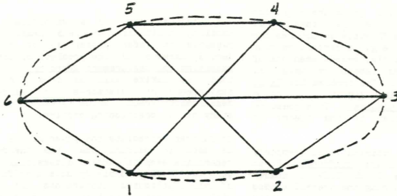
Figure 8. Pascal's Hexagon
