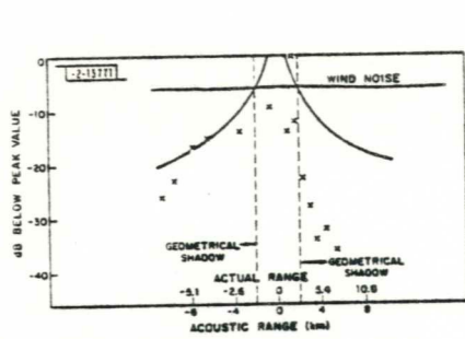
Fig. 16. Detection data for Ov-1D (altitude = 75 m, 0 dB = 88 dBa, windy conditions).
