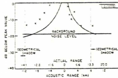
Fig. 15. Detection data for A-7 (altitude = 1020 m, 0 dB = 62 dBa).
