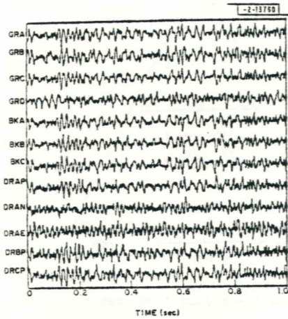
Fig. 5. Segment of A-7 acoustic digital data at an acoustic range of 8 km inbound.
