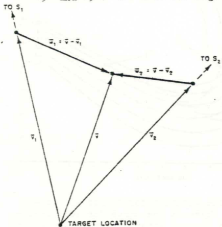
Fig. 4. \bar{v} is plane's apparent horizontal velocity. \bar{v}_1 is directed towards S_1 , \bar{v}_2 towards S_2 . If assumed height z = 0 , magnitude of \bar{v}_1 and \bar{v}_2 is speed of sound. \bar{w}_1 is directed along S_1 possible position curve, and \bar{w}_2 along S_2 possible position curve.
