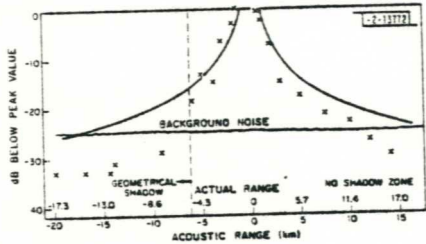
Fig. 17. Detection data for UH-1 (altitude = 300 m, 0 dB = 81 dBa).
