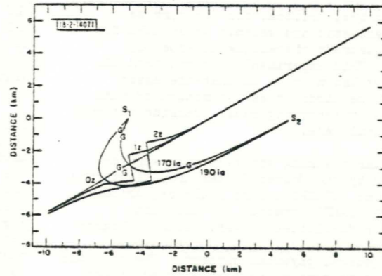
Fig. 7. Computed plane paths for assumed heights z = 0, 1, and 2 . Plane location is determined at times from -50 to +50 sec in 4 -sec increments. Region of linear ambiguity is also displayed.
