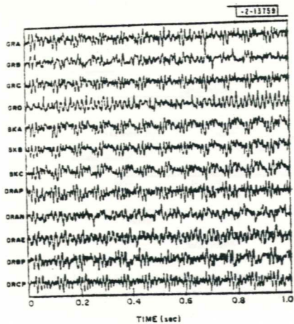
Fig. 4. Segment of UH-1 acoustic digital data at an acoustic range of 8 km inbound.
