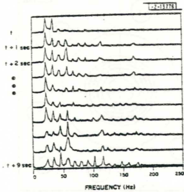
Fig. 21. Same as Fig. 19 for the U-1 circling at 5 km.
