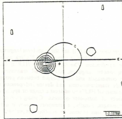
Fig. 32. High-resolution wavenumber spectrum for the A-7 at 8 km. True azimuth is \phi .
