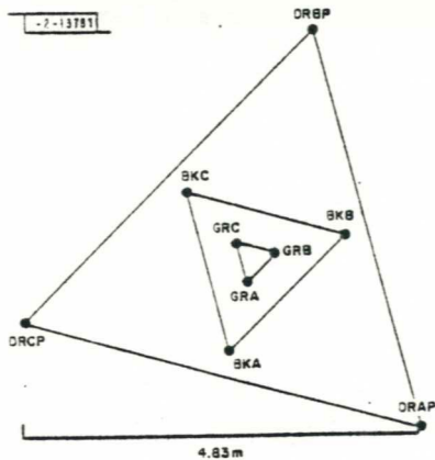
Fig. 27. Sensor stations used for array processing.
