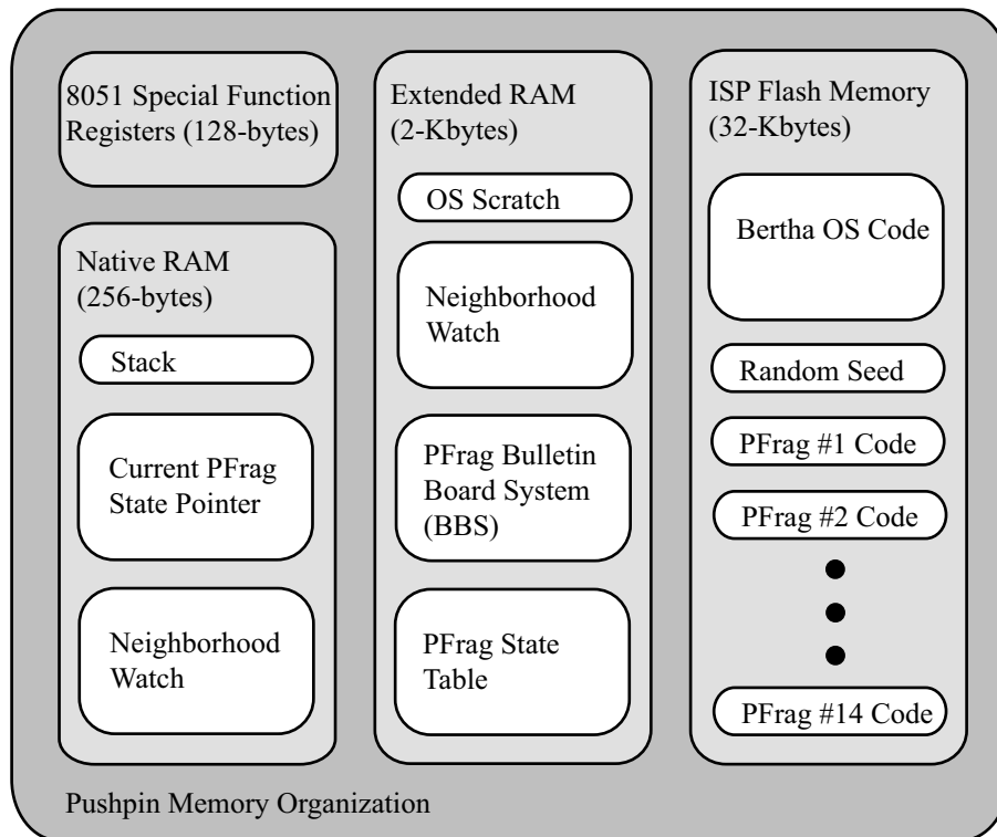
Fig. 4. A Pushpin's memory is carefully divided between process fragments and the operating system
