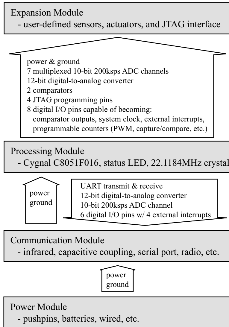
Fig. 3. The Pushpin hardware specification. The shaded boxes represent different hardware modules. The arrows represent resources that the module at the tail of the arrow provides to the module at the head of the arrow
