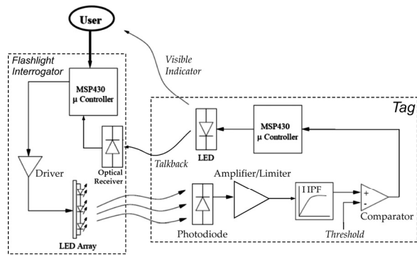
Figure 1: Block diagram of optical tag & interrogator
