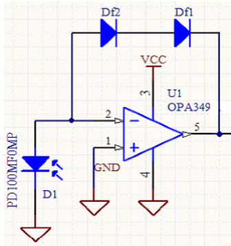
Figure 2: Photodiode amplifier/limiter circuitry
