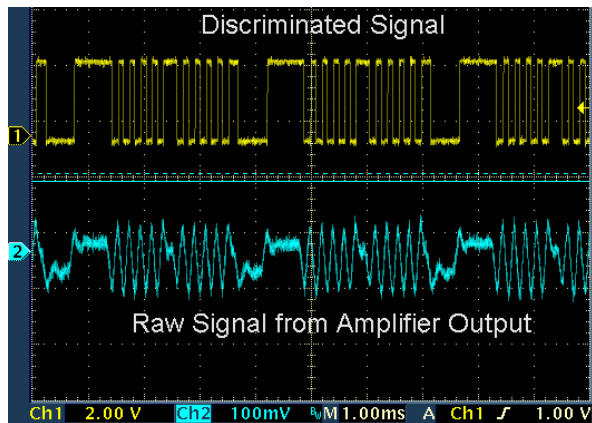
Figure 3: Noisy signal from amplifier (bottom) and recovered serial output from nanopower comparator (top) for the flashlight reader at 5 meter range
