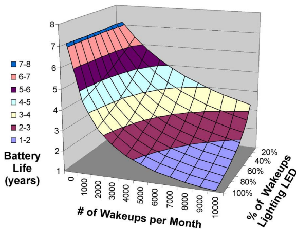
Figure 5: Tag Battery Life as a function of # wakeups and fraction that illuminate LED
