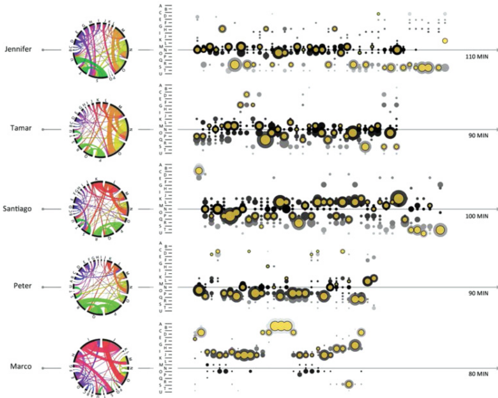
Fig. 17. The techniques detected for the five participants. Left: circular visualizations of the transition matrix between techniques, as a unique signature of the participants' work. The thickness of the connecting line is proportional to the number of transitions between these two states, while the colors are consistent between states of all users. Right: timeline of techniques with an averaging time window of 2.5 minutes.
